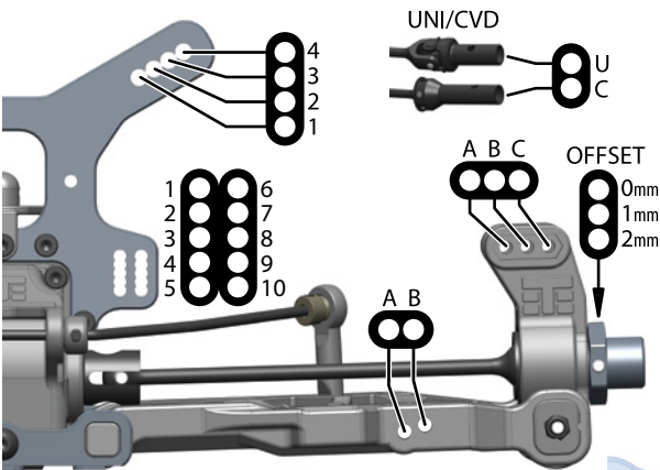
"C" Block: (Anti-Squat) (2° with center dot inserts)
